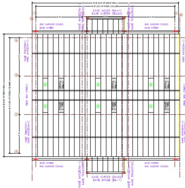
ROOF SHEETING PLAN
