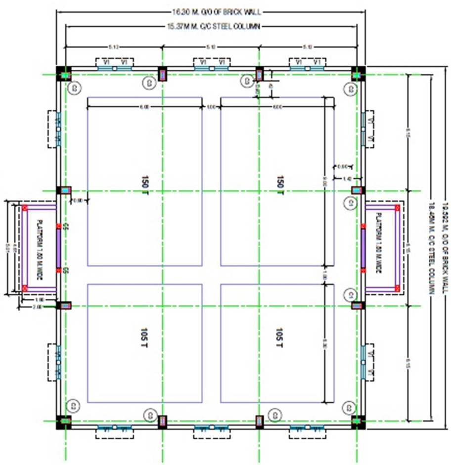
PLAN FOR 510 MT UNIT
